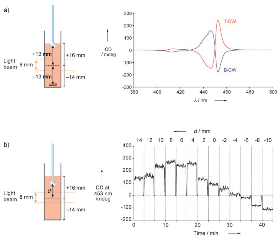
Figure 6. Circular dichroism (CD) spectra of a benzene solution (3.0 mL) of nanofibers of 1 ( 6.0 \times 10^{-6} M) at 20 °C in a 10 \times 10 \times 40 -mm 3 quartz optical cell under different stirring conditions. a) CD spectra upon top clockwise (T-CW) stirring using a \varnothing 8.0 \times 1.0 -mm 3 disk-shaped glass fin at 600 rpm (red) and bottom clockwise (B-CW) stirring using a \varnothing 2.0 \times 5.0 -mm 3 teflon-coated magnetic stirring bar at 900 rpm. The stirring positions for T-CW and B-CW were 13 mm above and below the center of an \varnothing 8.0 -mm-wide light beam, respectively. b) CD intensities at 453 nm upon rotary stirring at varying distances d from the light-beam. Whenever the stirring distance was changed, a shutter connected to the CD spectrometer was closed for 20 seconds.
